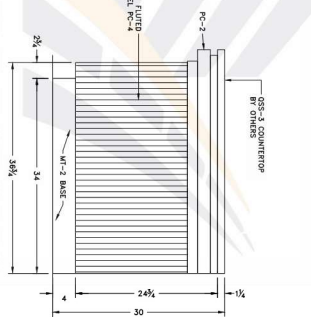
3 ELEVATION-LEASING A100 SCALE: 1"=1' REF. ARCH. B4/-803
